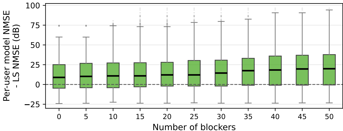
Per-user channel estimation model NMSE relative to LS
