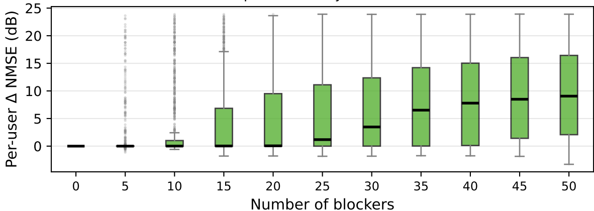
NMSE degradation of channel estimation model in the presence of dynamic blockers
