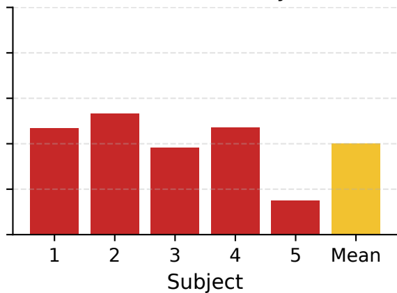
LOSO Accuracy
