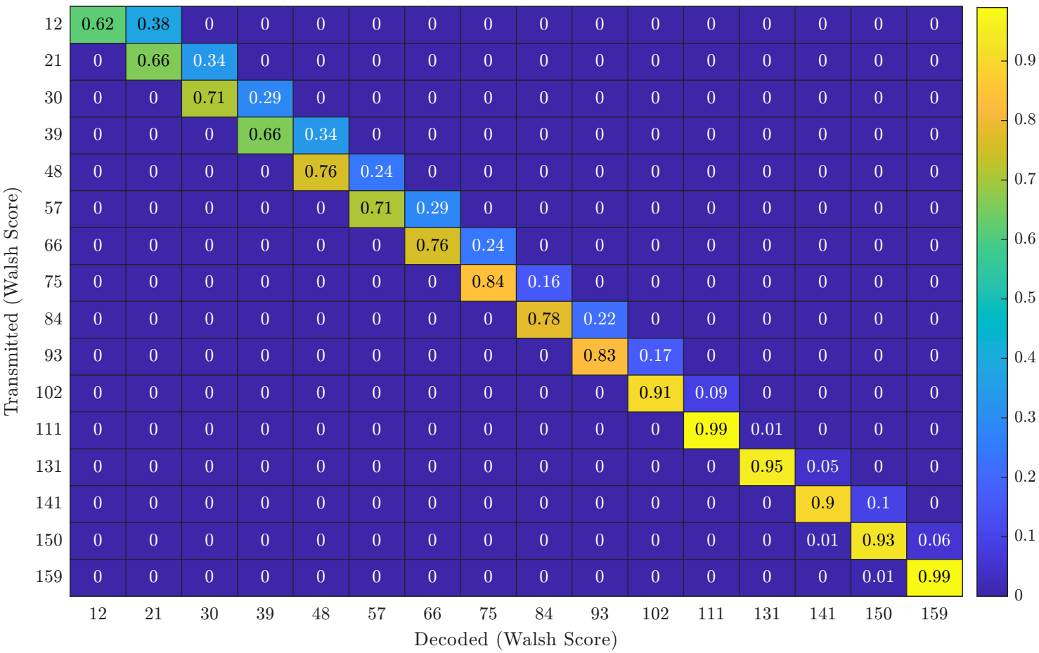
Heat Map for Backward Max-Gap, Percent Successfully Decoded, n = 512 , \omega_a = 512 Hz \omega_w = 10 Hz, 50 AWGN runs, 100 fade runs, r = -3 , P_c = 0.9900 , P_e = 0.9900
