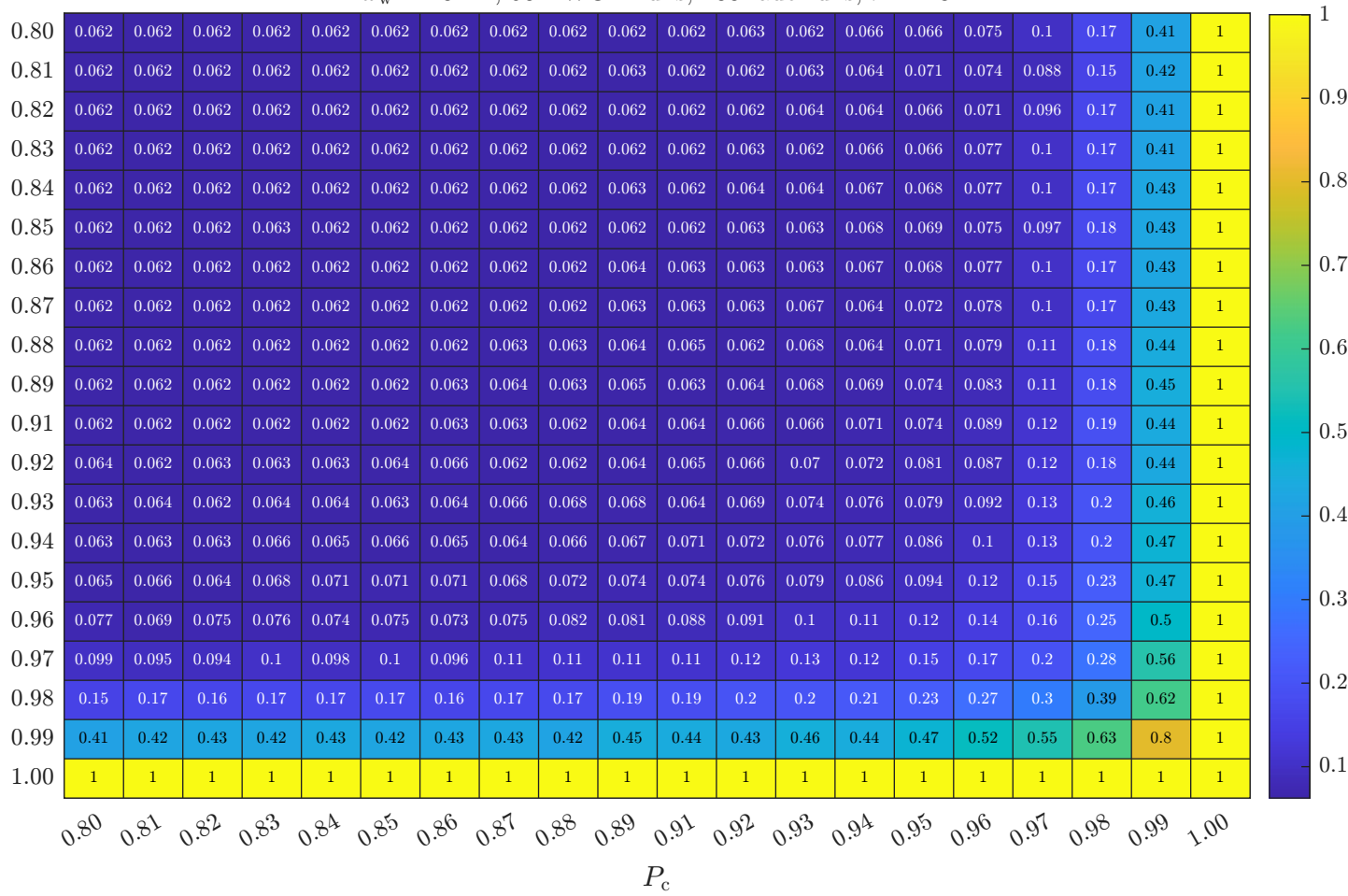
Heat Map for Backward Max-Gap, Percent Successfully Decoded, n = 512 , \omega_a = 512 Hz
