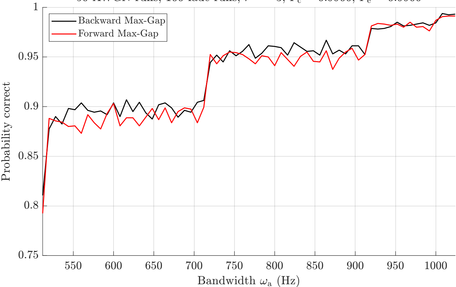
Probability correct vs. bandwidth, \omega_w = 10 Hz, n = 512 50 AWGN runs, 100 fade runs, r = -3 , P_c = 0.9900 , P_e = 0.9900
