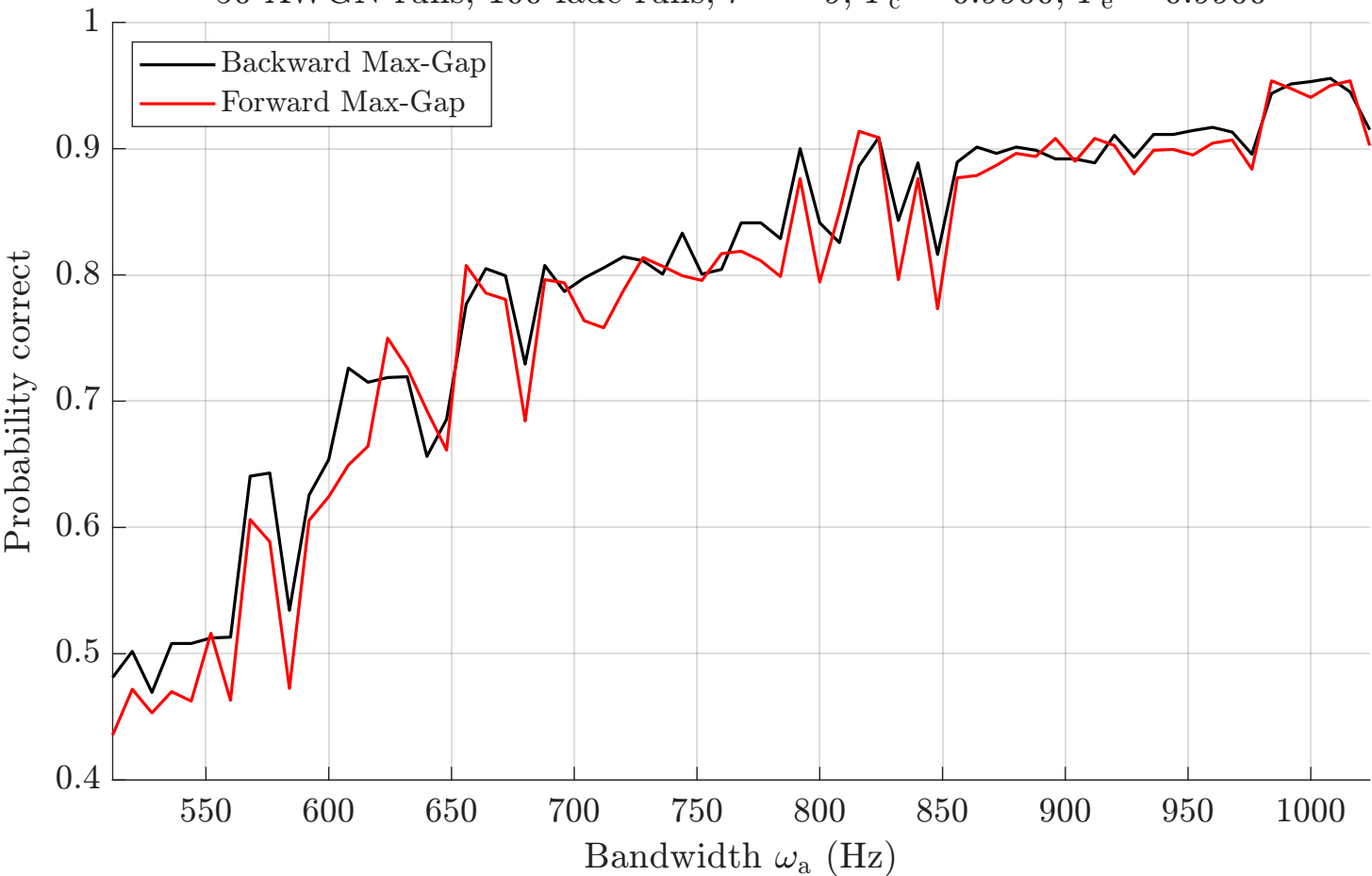
Probability correct vs. bandwidth, \omega_w = 10 Hz, n = 512 50 AWGN runs, 100 fade runs, r = -9 , P_c = 0.9900 , P_e = 0.9900
