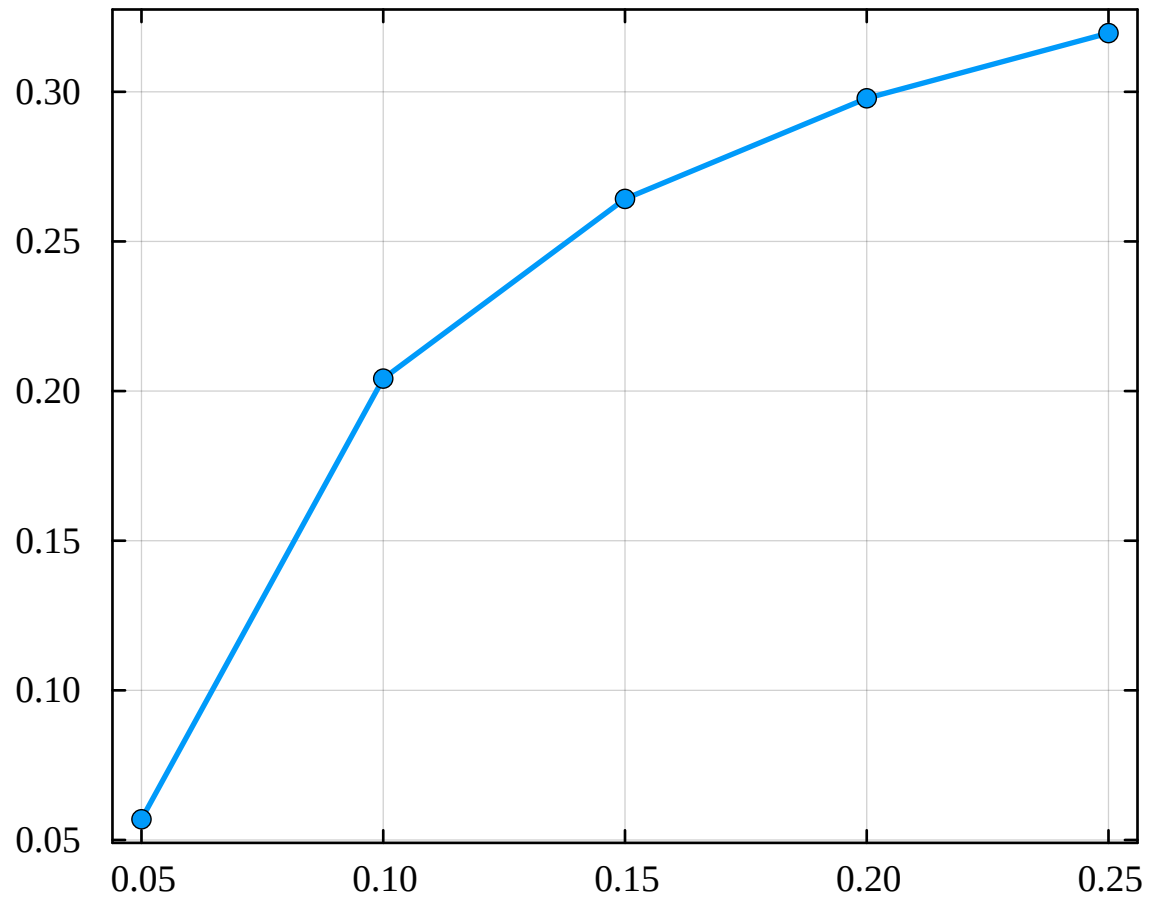
Relative error
