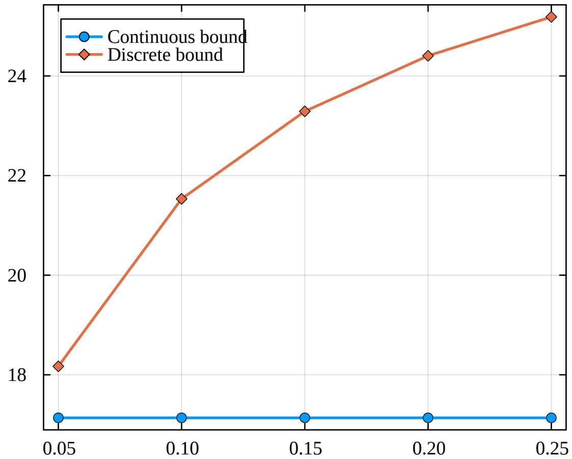
Mean Covariance
