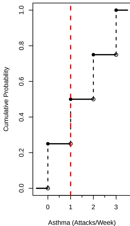
F(y) – CDF
