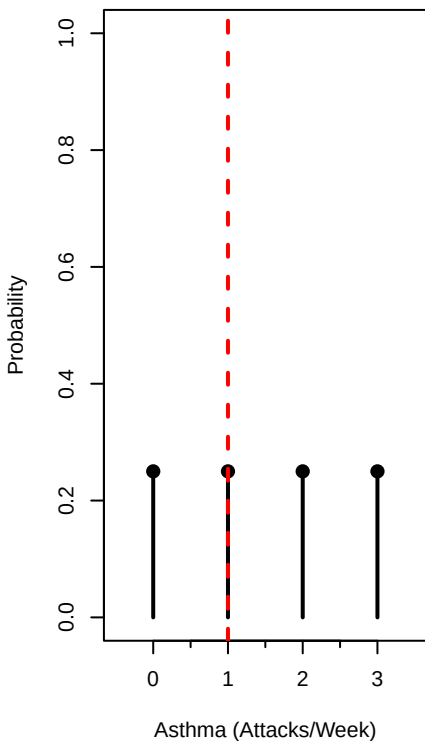
f(y) – PMF
