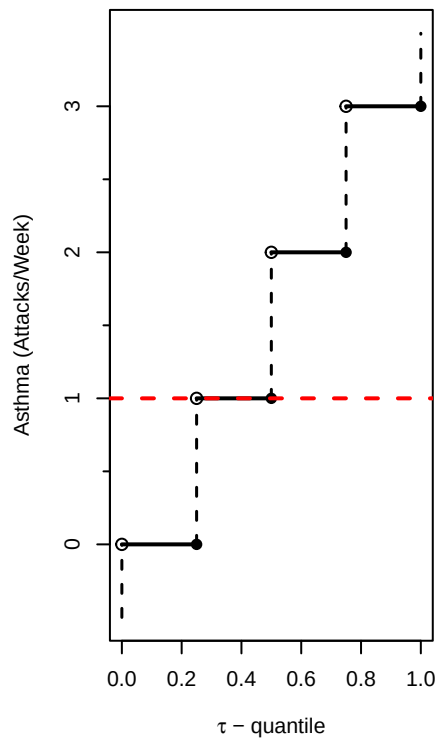
F^{-1}(\tau) – Quantile
