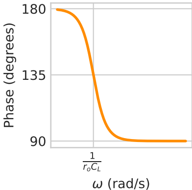
Phase Response
