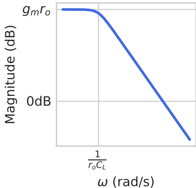
Magnitude Response
