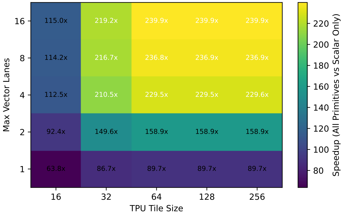
Speedup Heatmap @ 256b L1 Bandwidth
