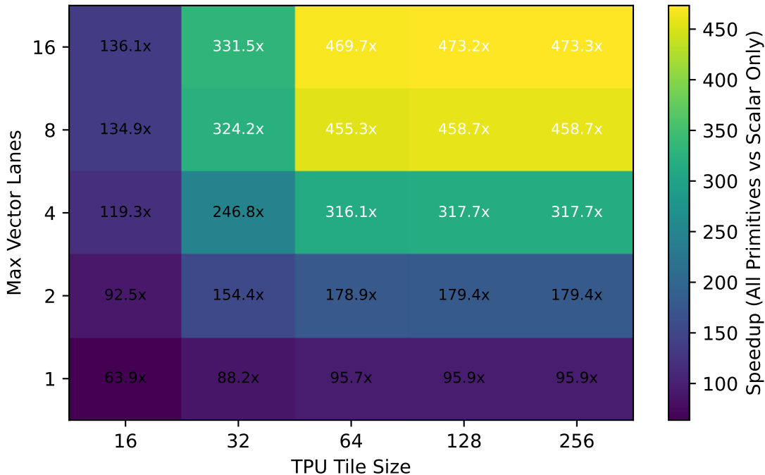
Speedup Heatmap @ 512b L1 Bandwidth
