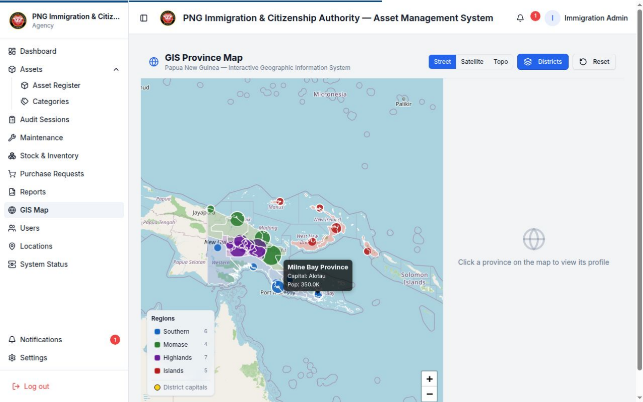
Figure A4 — GIS Province Map: interactive Leaflet map of all 22 PNG provinces with district overlays, basemap selector and per-province asset / population profile (Street / Satellite / Topo).
