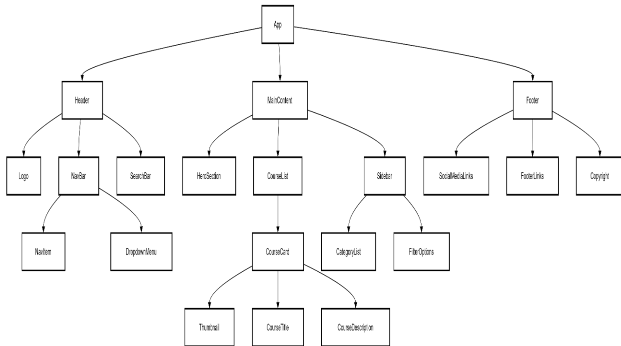
Figure 4: Component Hierarchy Diagram
