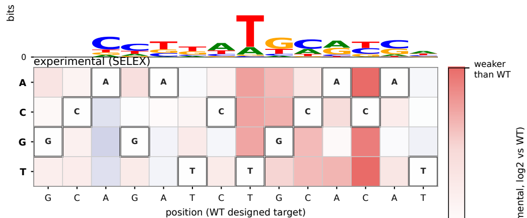
2 DBP035 — TFScope predicted (logo)
