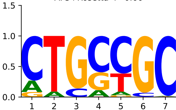
AF3+Rosetta r=0.66
