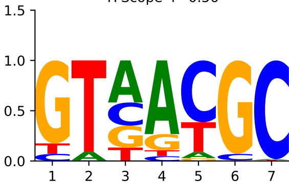
TFScope r=0.56
