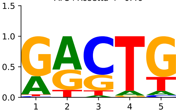
AF3+Rosetta r=0.46
