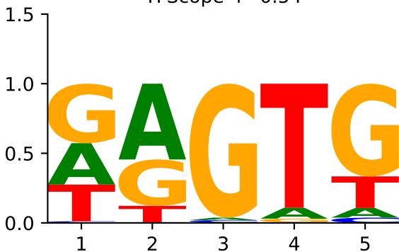
TFScope r=0.54
