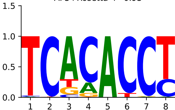
AF3+Rosetta r=0.93
