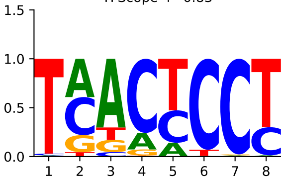
TFScope r=0.83
