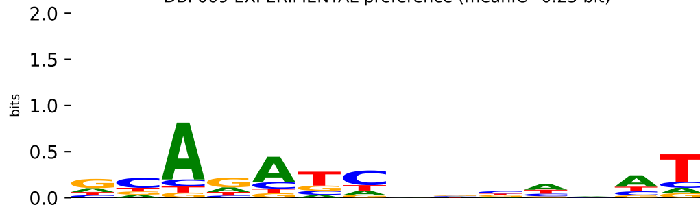
DBP035 EXPERIMENTAL preference (meanIC=0.32 bit)
