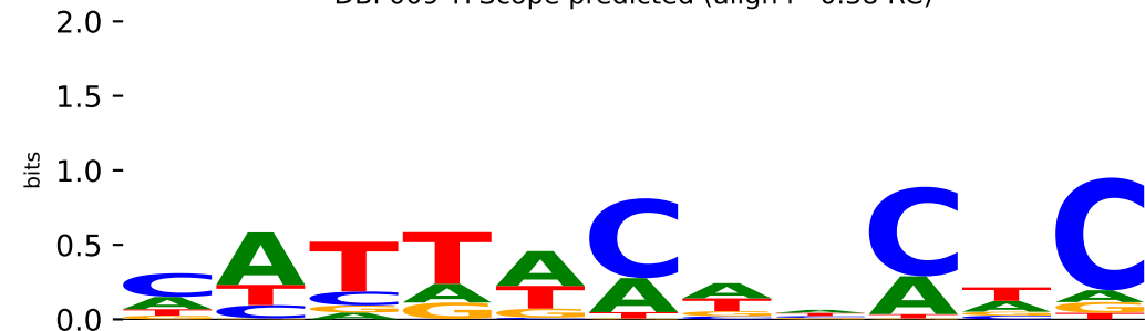
DBP035 TFScope predicted (align r=0.38)
