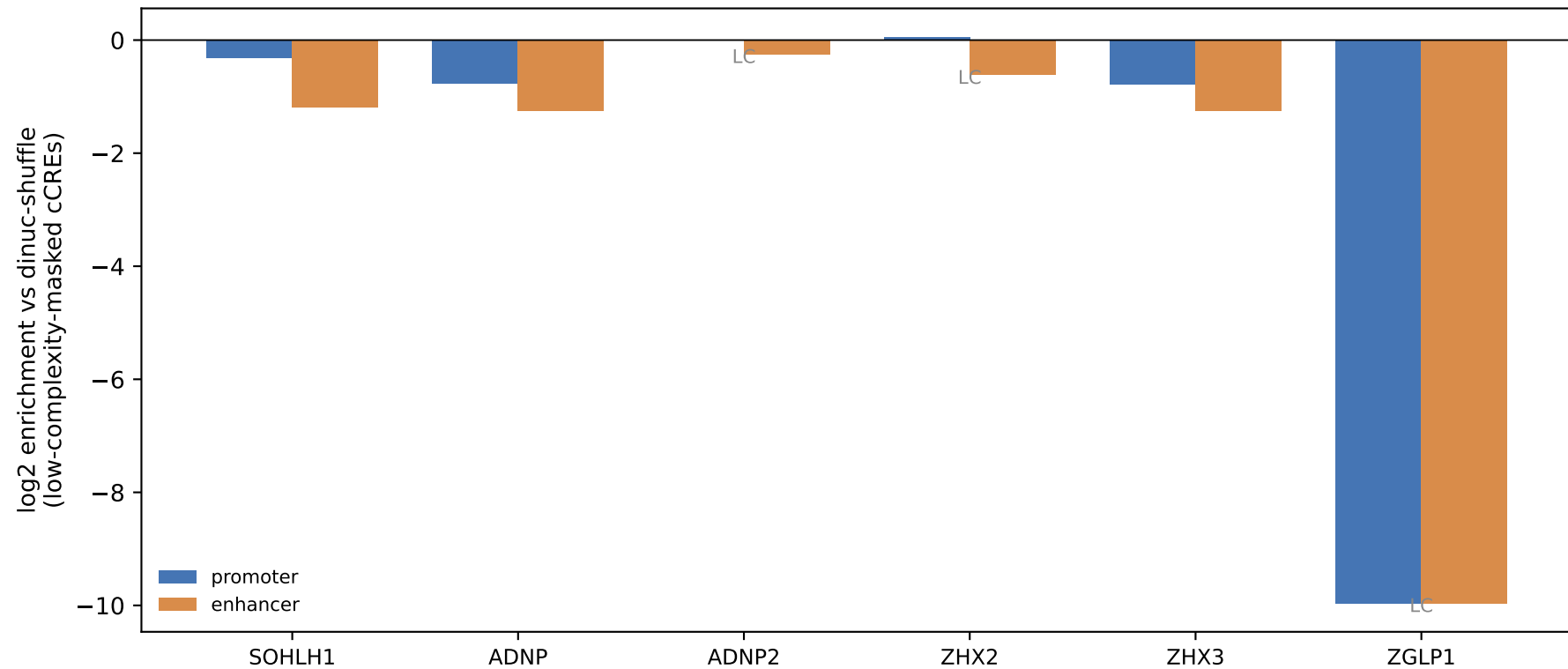
Fig 3b-c (MoE-base) — low-complexity-masked; LC = poly-A/low-complexity motif (unreliable)
