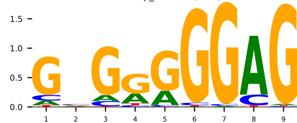
GT 4r2p_A WT1 (K=9)
