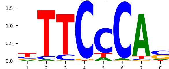
GT 6wqu_C RBPJ (K=8)
