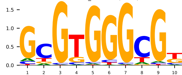
GT 4r2d_A EGR1 (K=10)
