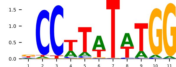
GT 1srs_B SRF (K=11)
