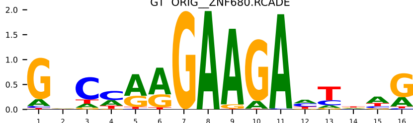
GT ORIG_ZNF534.H13CORE.0.P.C
