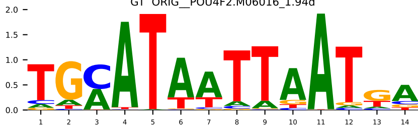
GT ORIG_POU4F2.M06016_1.94d
