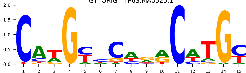
GT ORIG_TP63.MA0525.1
