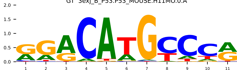
GT ORIG_ZNF398.MEME
