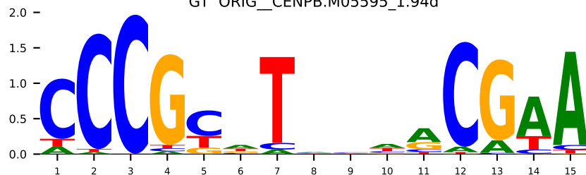
GT 6pax_A_PAX6.MA0069.1
