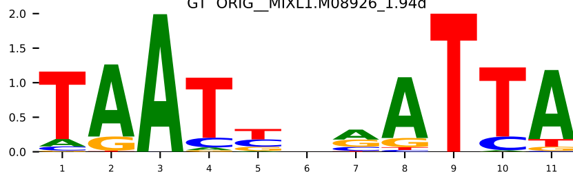
GT ORIG_TBX5.M06173_1.94d
