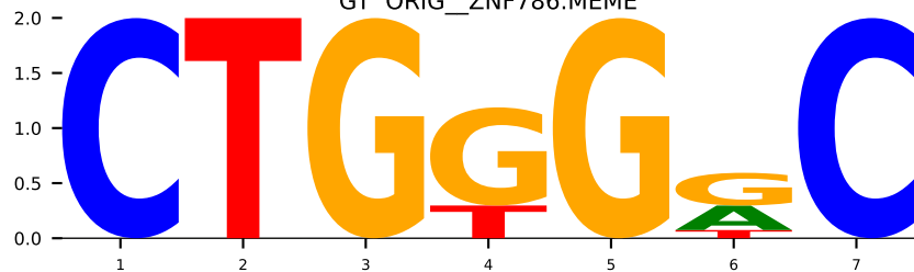
GT ORIG_POU1F1.MA0784.2
