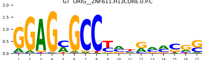
GT ORIG_ZNF611.H13CORE.0.P.C
