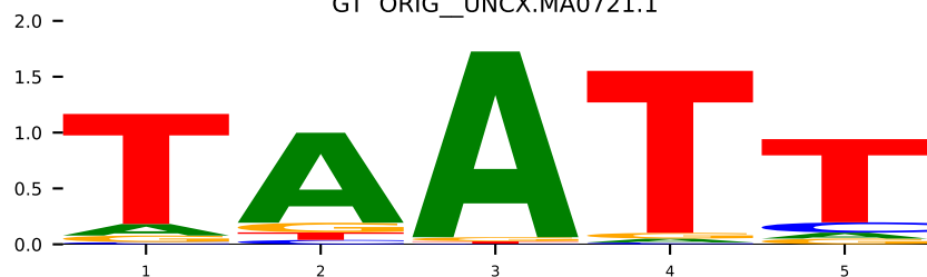
GT ORIG_POU3F3.H13CORE.1.P.C
