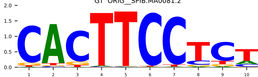
GT 1cqt_B_POU2F1.MA0785.1
