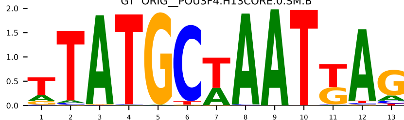
GT ORIG_POU3F4.H13CORE.0.SM.B
