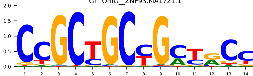
GT ORIG_ZNF85.H13CORE.1.P.B
