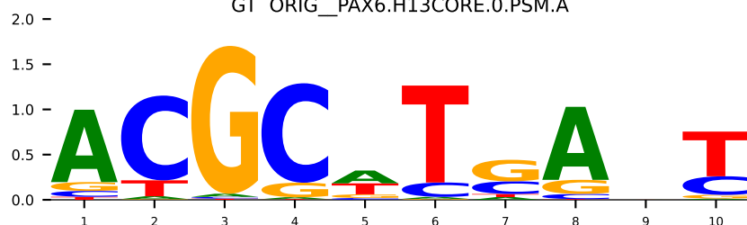
GT ORIG_PAX6.H13CORE.0.PSM.A
