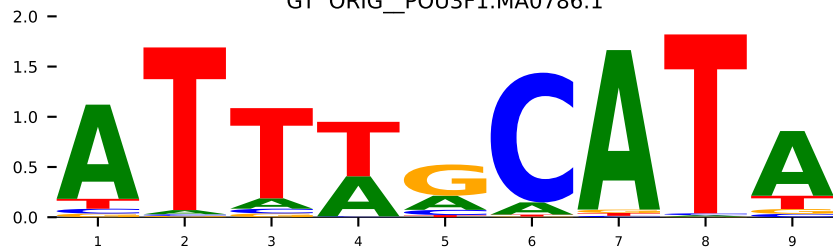
GT ORIG_POU4F1.M09911_1.94d
