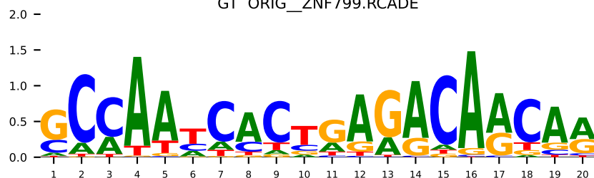
GT ORIG_ATOH1.H13CORE.0.PB
