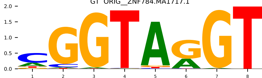
GT ORIG_POU3F2.M06009_1.94d
