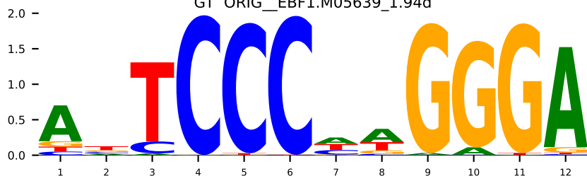
GT ORIG_EBF1.MA0154.3
