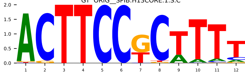
GT 1gt0_C_POU2F1::SOX2.MA1962.1
