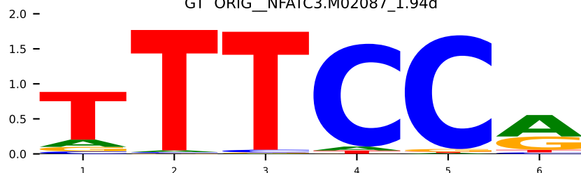
GT ORIG_NFATC3.MA0625.1
