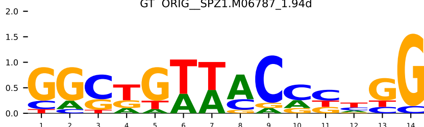
GT ORIG_SPZ1.M06787_1.94d
