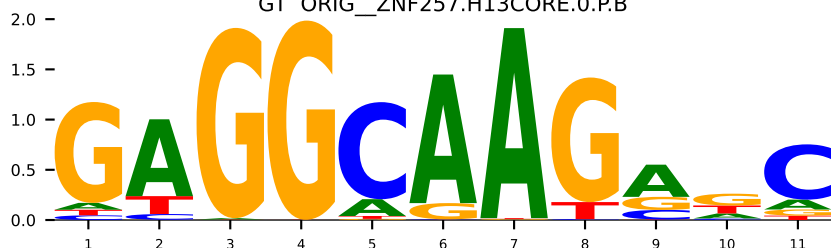
GT ORIG_ZNF257.H13CORE.0.P.B
