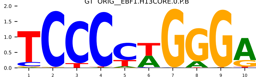
GT ORIG_NR1I3.MA1534.1
