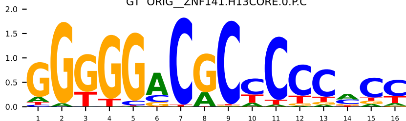
GT 1p7h_L_NFATC2.MA0152.1
