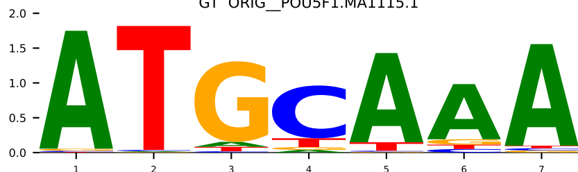
GT ORIG_POU5F1.MA1115.1
