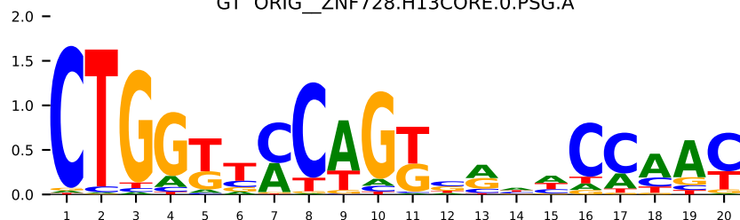
GT ORIG_ZNF611.H13CORE.1.P.C
