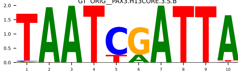
GT 7ogs_F_IRF4.MA1419.1
