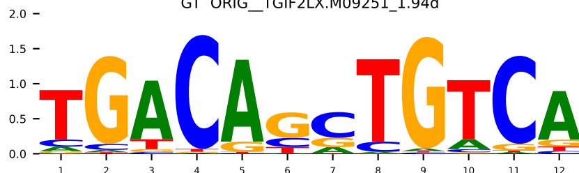
GT ORIG_TGIF2LX.MA1571.1
