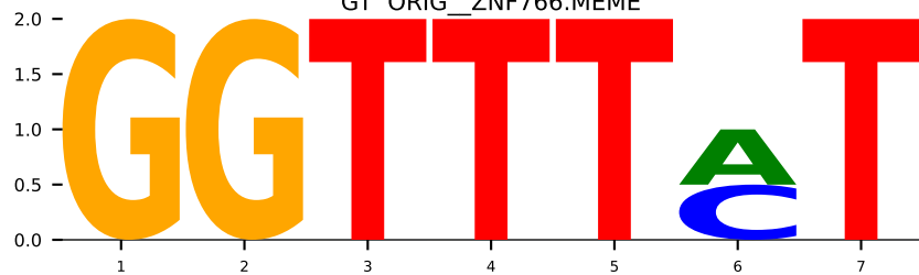
GT ORIG_ZNF766.MEME
