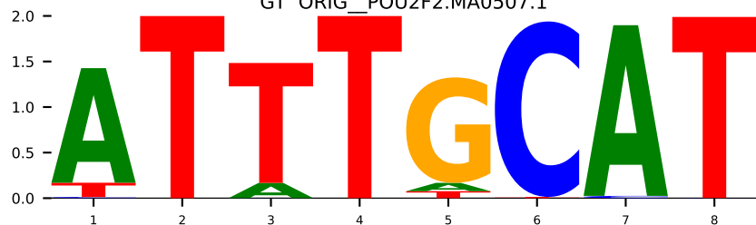
GT ORIG_NFATC3.H13CORE.1.P.C
