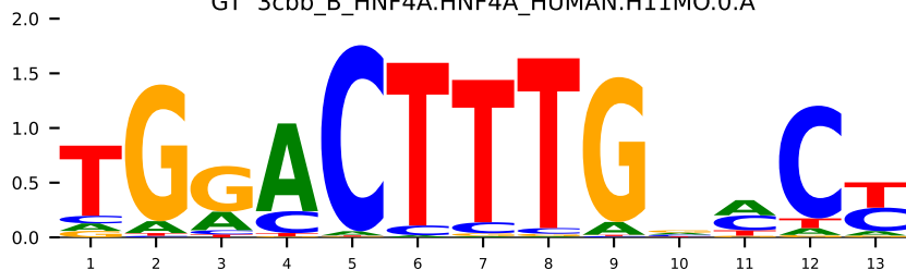
GT 3cbb_B_HNF4A.HNF4A_HUMAN.H11MO.0.A
