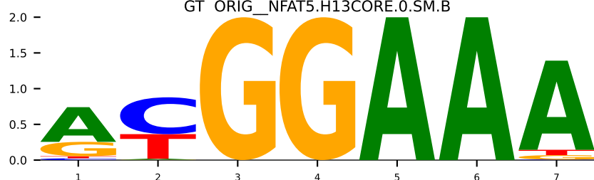
GT ORIG_NFAT5.H13CORE.0.SM.B
