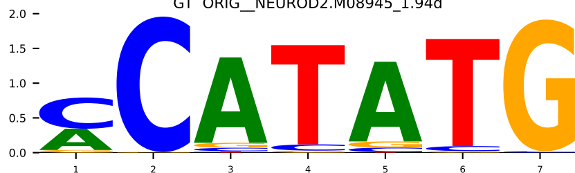
GT ORIG_FOXK1.MA0852.2
