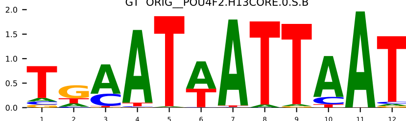
GT 3cbb_A_HNF4A.MA1494.1
