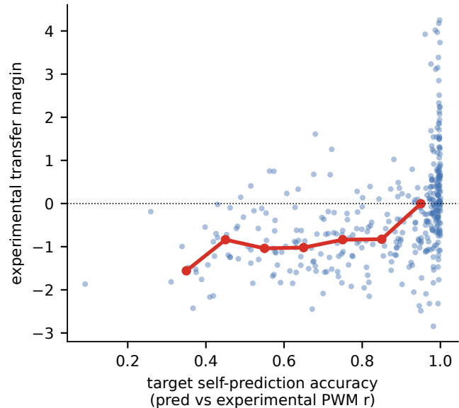
c Transfer \propto self-prediction \rho=0.55 ( p=3e-31 , n=375 )
