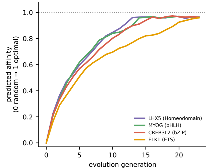
a In-silico SELEX recovers consensus
