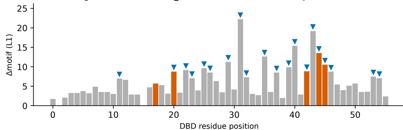
b C2H2 zinc finger: ZBTB7A (C2H2_medium) AUROC=0.83, top-20 recovers 4/6 contacts
