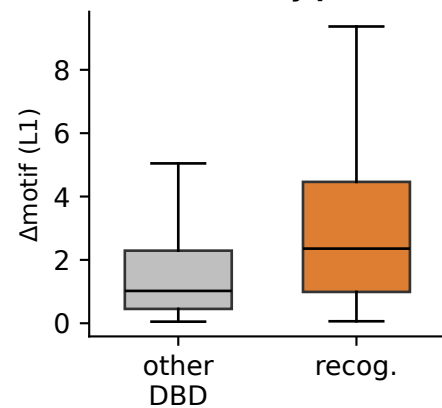
d recog. > other DBD (Mann-Whitney p=2\text{e-}32 )
