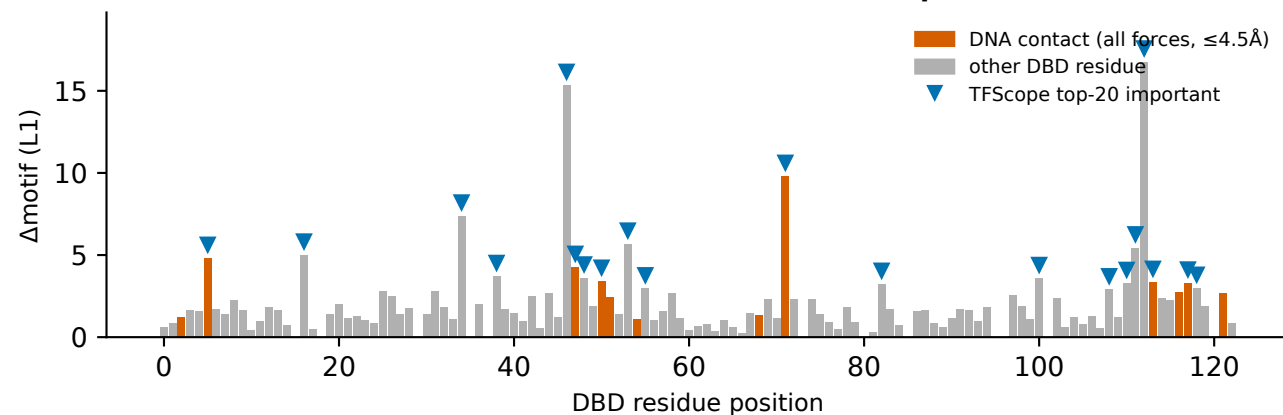
a homeodomain: DUX4 (Homeodomain) AUROC=0.76, top-20 recovers 6/12 contacts
