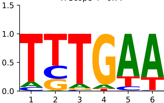
TFScope r=0.77
