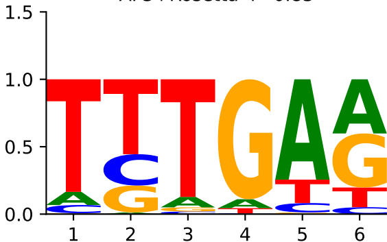
AF3+Rosetta r=0.83
