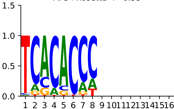
AF3+Rosetta r=0.53
