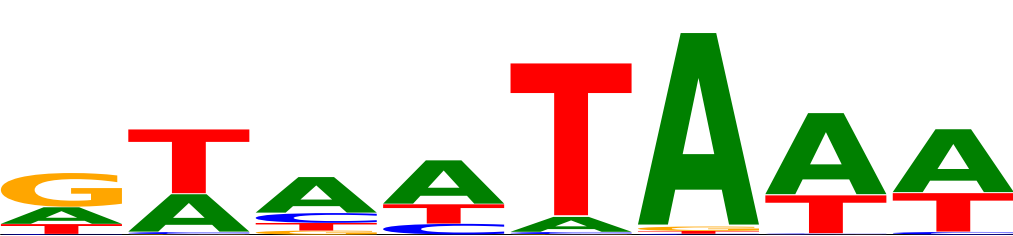
4. all-DBD (6 domains) | gate core GAAATAAA GC 0.11 LC 0.75 r=0.50
