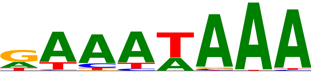
5. full sequence | gate core GAAATAAA GC 0.11 LC 0.75 r=0.48
