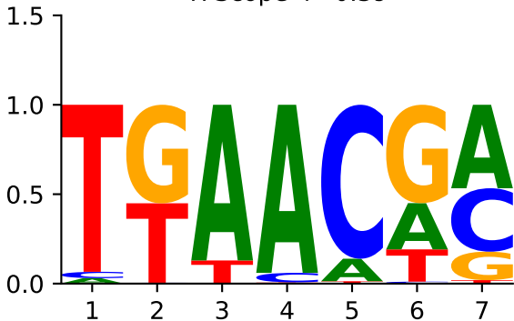
TFScope r=0.39
