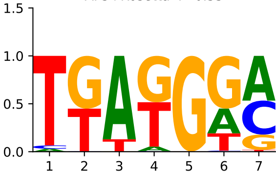
AF3+Rosetta r=0.55
