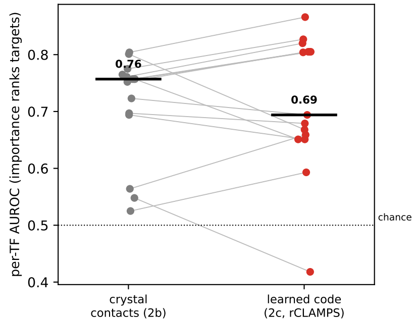
b Recovered across two independent ground truths
