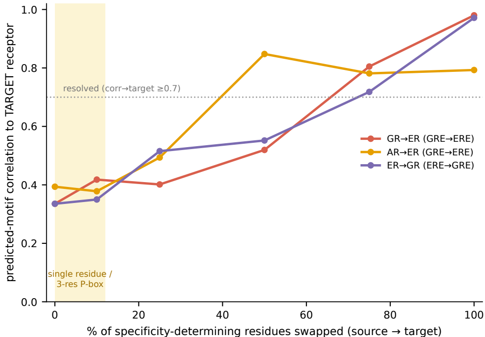
Sequence-only resolution scales with the size of the determinant change
