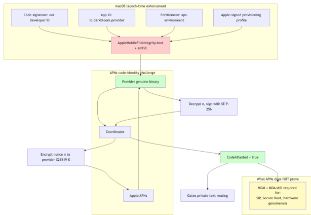
Figure 2: APNs code-identity attestation. AMFI (AppleMobileFileIntegrity.kext) enforces code signature, App ID, and aps-environment entitlement at launch, so only the genuine Darkbloom binary can register for our push topic. The coordinator pushes an encrypted nonce to that topic; the provider decrypts it with its bound X25519 key and returns a Secure Enclave signature, proving the WebSocket session is backed by genuine code holding the decryption key. MDM and MDA remain required for SIP, Secure Boot, and hardware provenance.
