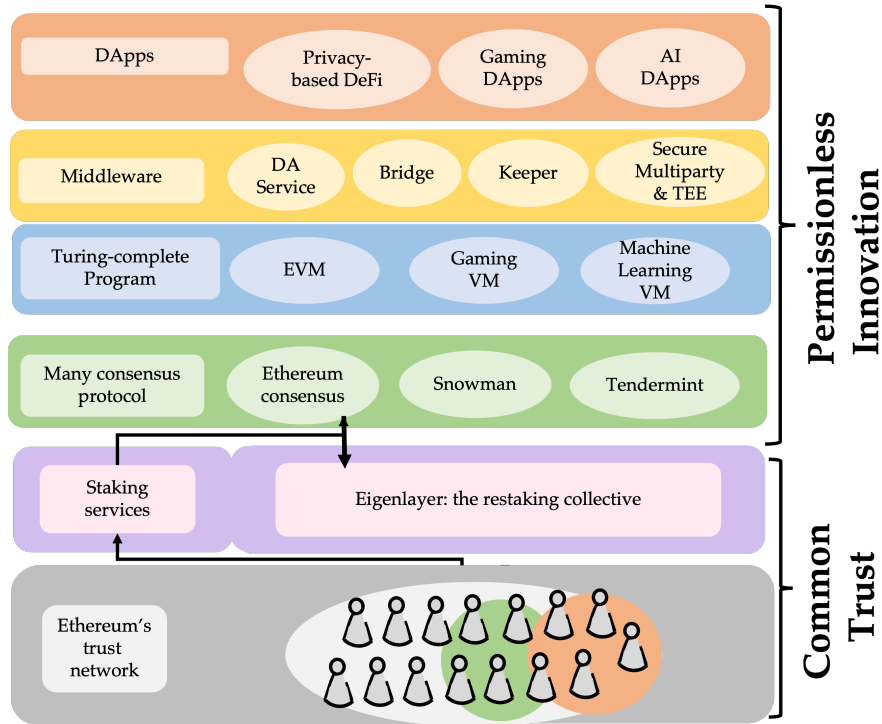
Figure 4: With EigenLayer, permissionless innovation permeates deeper into the blockchain stack.
