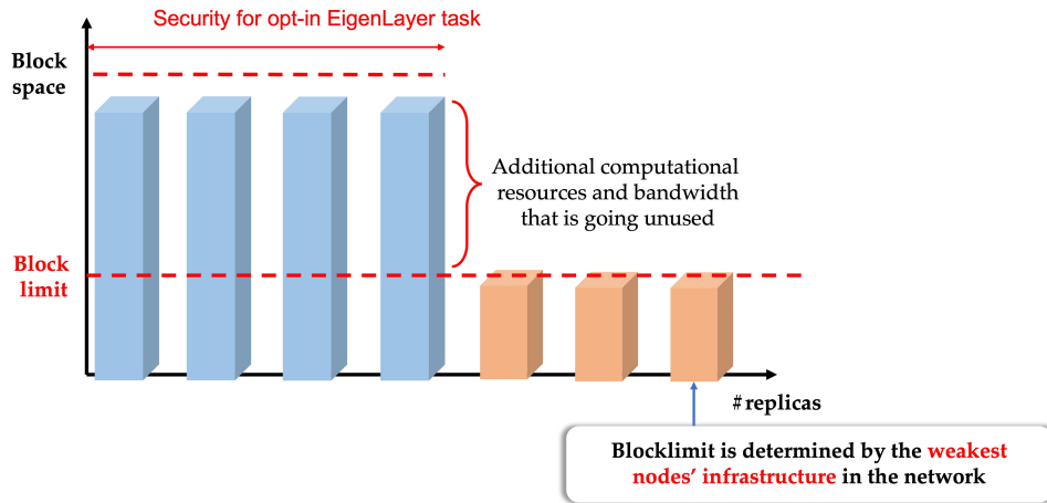
Figure 7: Blockspace is the most valuable commodity in blockchains [11]. In today’s ecosystem, blocklimit on this blockspace is determined by weakest validator’s infrastructure. This limit arises from Ethereum’s focus on decentralization. However, EigenLayer can leverage the extra capabilities of validators with additional resources to provide guarantees of cryptoeconomic security to applications that desire them.
