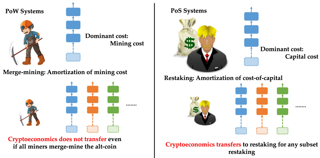
Figure 6: Merge mining vs. restaking.
