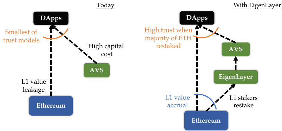
Figure 1: Comparing the ecosystem of actively validated services today and with EigenLayer.
