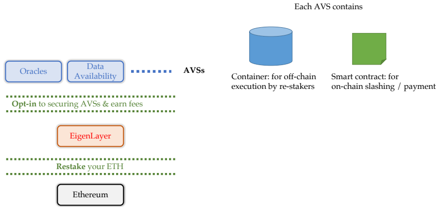
Figure 2: Launching an AVS on top of EigenLayer requires deploying an off-chain container that operators must download, and an on-chain contract that specifies the terms of slashing and payment.
