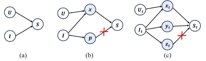
Fig. 2. Causal graphs of: (a) traditional models; (b) general debiasing models; and (c) our proposed CDSRec model. U , user; I , item; S , prediction result; p , popularity; x , personalized demand factors; y , inherent quality factors; and z , external interference factors.
