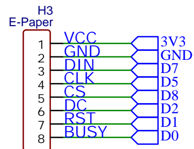
E-paper
