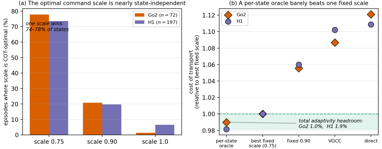
Figure 4: The paper’s central finding, on paired-successful episodes (identical initial states). (a) The COT-optimal command scale is nearly the same in every state: a single scale is optimal in 74–78% of episodes on both robots, so there is little for a state-conditioned controller to specialize to. (b) Cost of transport relative to the best single fixed scale (= 1): an omniscient per-state oracle that picks the best scale for every episode lies only 1.0% (Go2) and 1.9% (H1) below that fixed scale; the entire shaded band is the total adaptivity headroom available to any state-conditioned method. VGCC and direct control sit above the fixed scale, not because they model the policy poorly but because the headroom they compete for is nearly empty.
