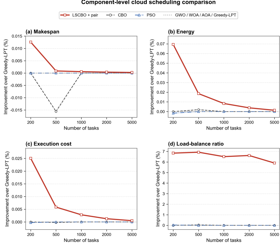
Fig. 6 Component-level cloud scheduling comparison across task scales. Positive values indicate component-wise improvement over Greedy-LPT. The figure separates makespan, energy, execution cost, and LBR to show that the main visible change comes from load-balance refinement, while physical-cost changes remain small. GWO, WOA, and AOA are grouped with Greedy-LPT because their formal traces are identical under the reported protocol.
