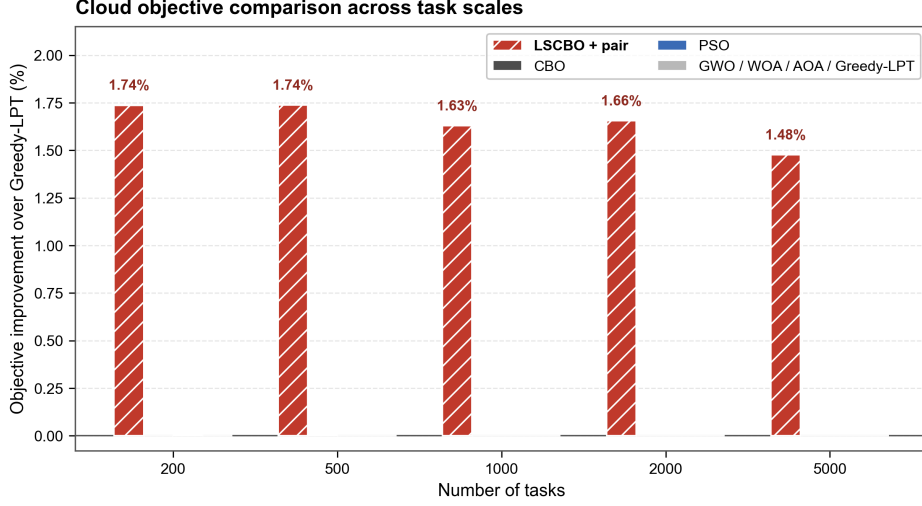
Fig. 5 Scale-wise cloud objective comparison. Bars show paired mean objective improvement over Greedy-LPT across 30 seeds. Positive values indicate a lower reference-normalized scalar objective. GWO, WOA, and AOA are grouped with Greedy-LPT because their formal traces coincide with the deterministic warm-start schedule.
