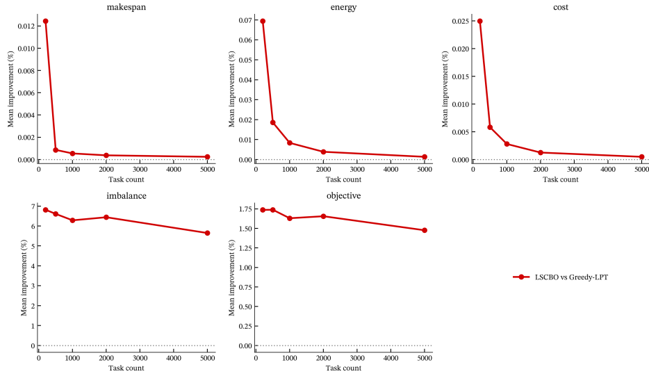
Fig. 5 Mean component-wise improvement of LSCBO over Greedy-LPT. The zero line denotes equality; positive values favor LSCBO.
