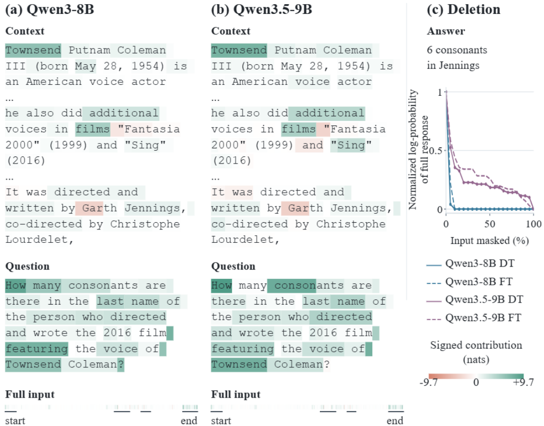
Figure 4: Signed evidence across a multi-hop question. (a,b) The MoreHopQA input links Townsend Coleman to Sing , Garth Jennings, and his surname’s consonants. (c) Normalized log-probability of the full fixed response plus EOS, comparing each model’s DT with its own one-hop FT baseline. Model colors, method line styles, and per-model normalization follow Figure 3. Both heatmaps share the signed scale within this example.
