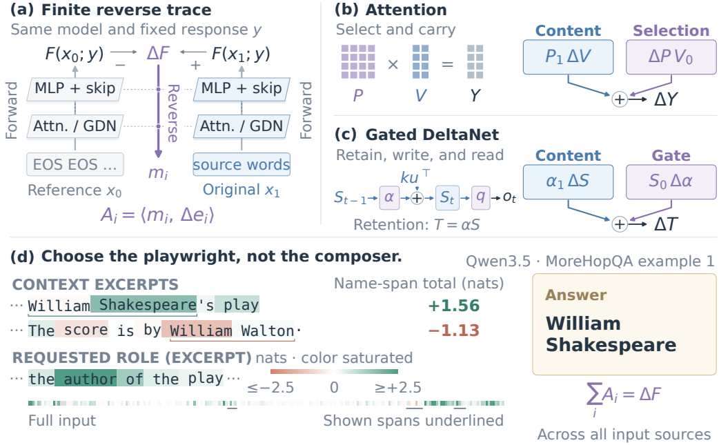
Figure 1: DeltaTrace follows both content and control. (a) Gray arrows show two forward executions with the same fixed response y , defining \Delta F = F(x_1; y) - F(x_0; y) . The purple arrow shows one reverse traversal using finite-difference rules: the resulting coefficients m_i map embedding differences \Delta e_i to signed source contributions A_i . (b,c) Attention and gated memory share a content/control allocation. The memory example expands retention, T = \alpha S , with S the previous state. The operators are schematic. (d) Actual Qwen3.5 scores from MoreHopQA development example 1 assign positive credit to the playwright’s name and negative credit to the composer’s name. Backgrounds show token scores; annotations sum only the indicated name spans. One linear color scale is explicitly saturated at \pm 2.5 nats. Ellipses mark omitted text. The requested role and identified playwright are shown; attribution targets the complete stored response plus EOS. Conservation refers to all input sources.
