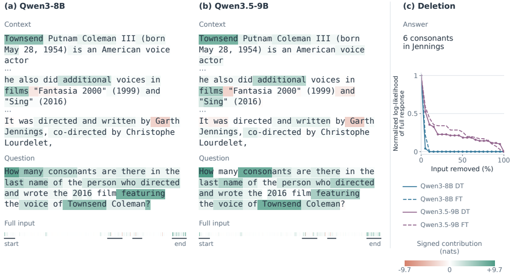
Figure 4: Signed evidence across a multi-hop question. (a,b) The MoreHopQA input links Townsend Coleman to Sing , Garth Jennings, and his surname’s consonants. (c) Normalized log-likelihood of the entire fixed response plus EOS, comparing each model’s DT with its own one-hop FT baseline. Model colors, method line styles, and per-model normalization follow Figure 3. Both heatmaps share the signed scale within this example.
