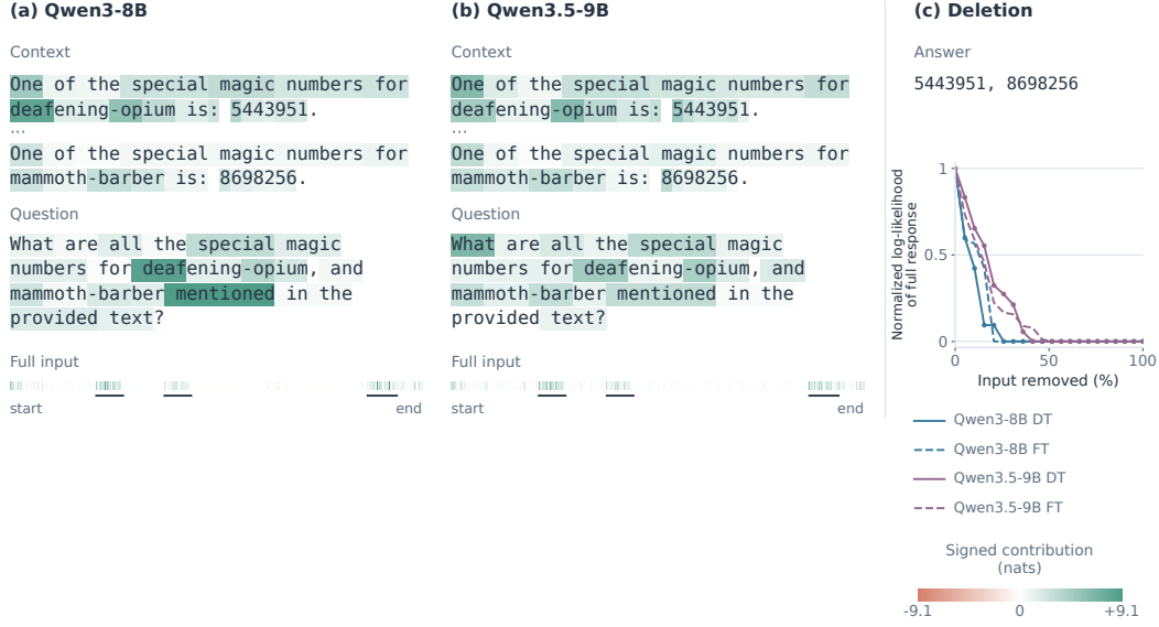
Figure 3: Signed evidence for retrieving two numbers. (a,b) The same niah_mq-q2 input on Qwen3-8B and Qwen3.5-9B; teal and coral show positive and negative DT contributions in nats. Marks locate excerpts. (c) Each model’s DT (solid) and one-hop FT (dashed) curves show the normalized log-likelihood of the entire fixed response plus EOS under 20-step deletion. Color identifies the model. The released normalization uses that model’s full-input and fully-deleted scores, clipping and a cumulative minimum. DT deletion uses positive ranking. Answer summarizes the full stored response.
