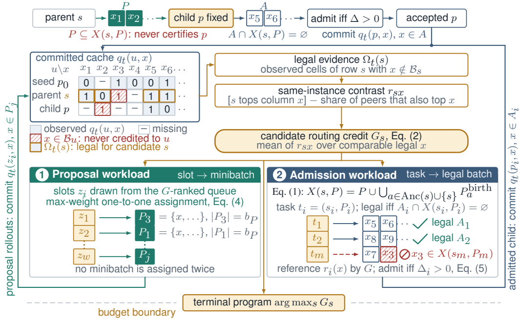
Figure 1: Provenance-constrained evidence routing in COMPASS. A child p is proposed from parent s by minibatch P and certified on an admission batch A drawn outside the recursive exclusion set X(s, P) (Equation (1)); accepted observations enter the committed cache q_t(u, x) . For candidate s , only cache entries outside its lineage birth set \mathcal{B}_s (unhatched) are legal evidence \Omega_t(s) ; each is contrasted with the peers observed on the same instance, and the mean contrast is the routing credit G_s (Equation (2)). G_s then allocates proposal slots to distinct minibatches and references for each legal admission batch, and selects the terminal program. Red marks an instance inside the birth provenance of the lineage in question.
