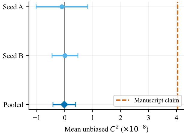
Simeck-48, 17 rounds
