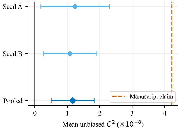
Simeck-48, 14 rounds
