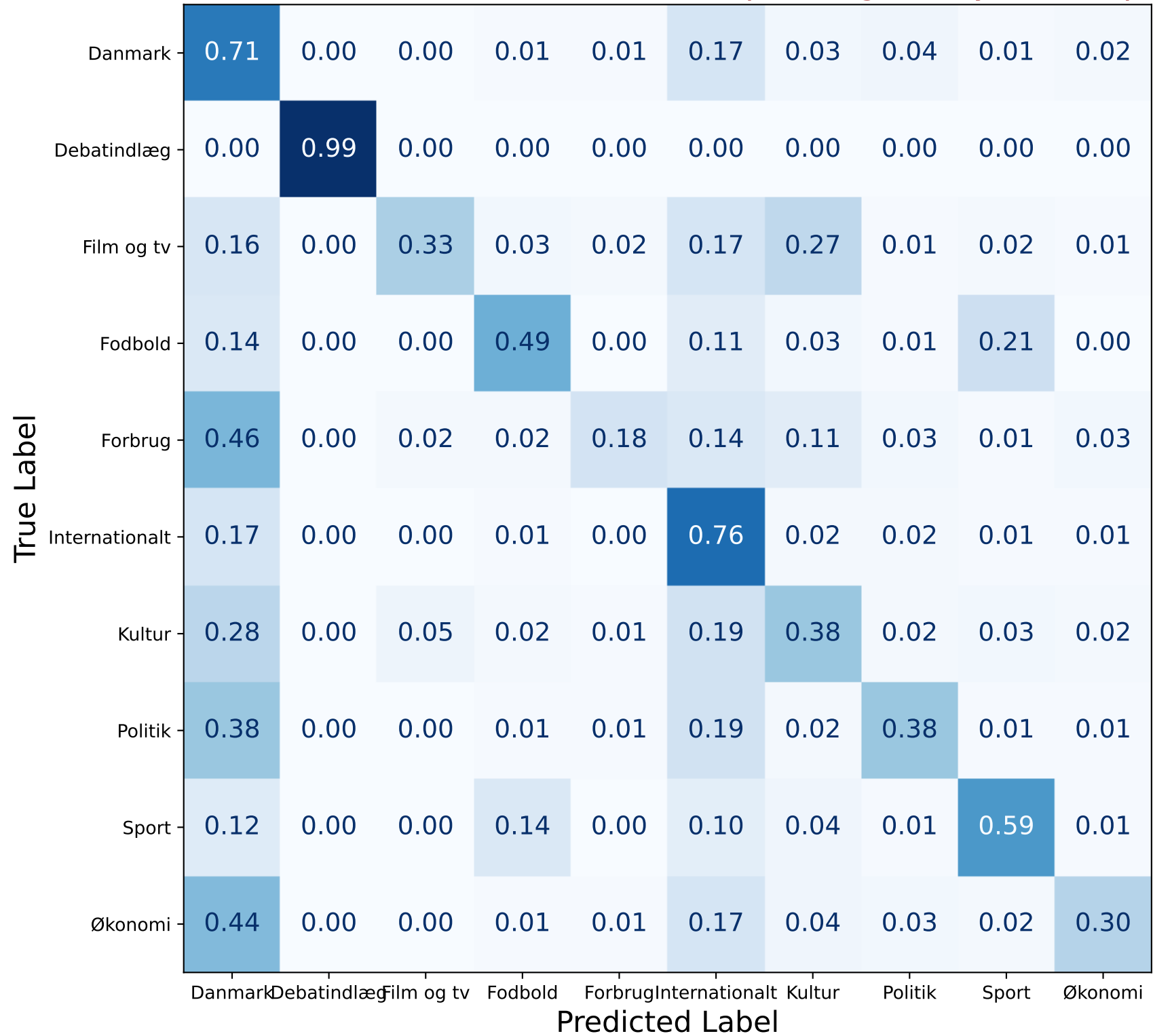
Multiclass Confusion Matrix Article Topics Trigram PyTorch Top 10
