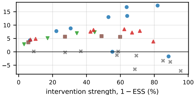
(a) Synthetic, hard region
