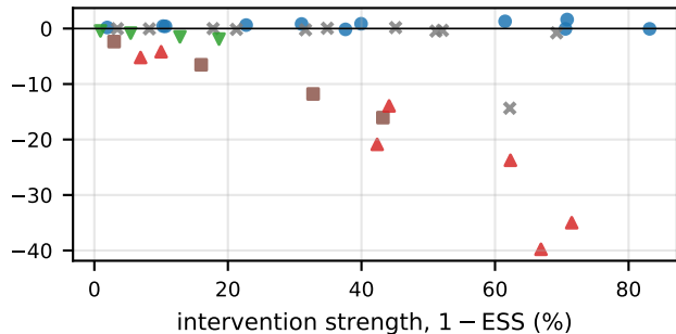
(b) California housing
