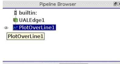
Figure 36: Hide/Show indicator
