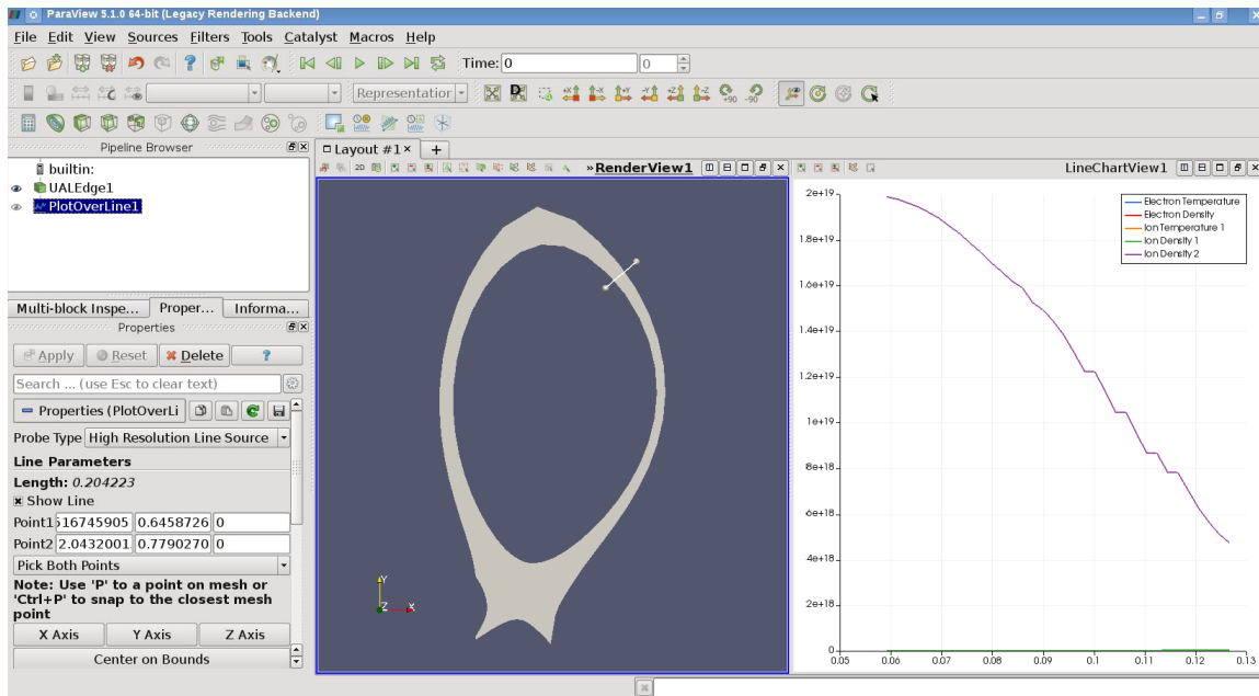
Figure 30: Chart example
