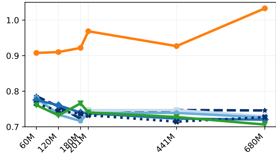
Model: ResNet
