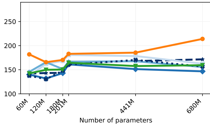
Model: ResNet
