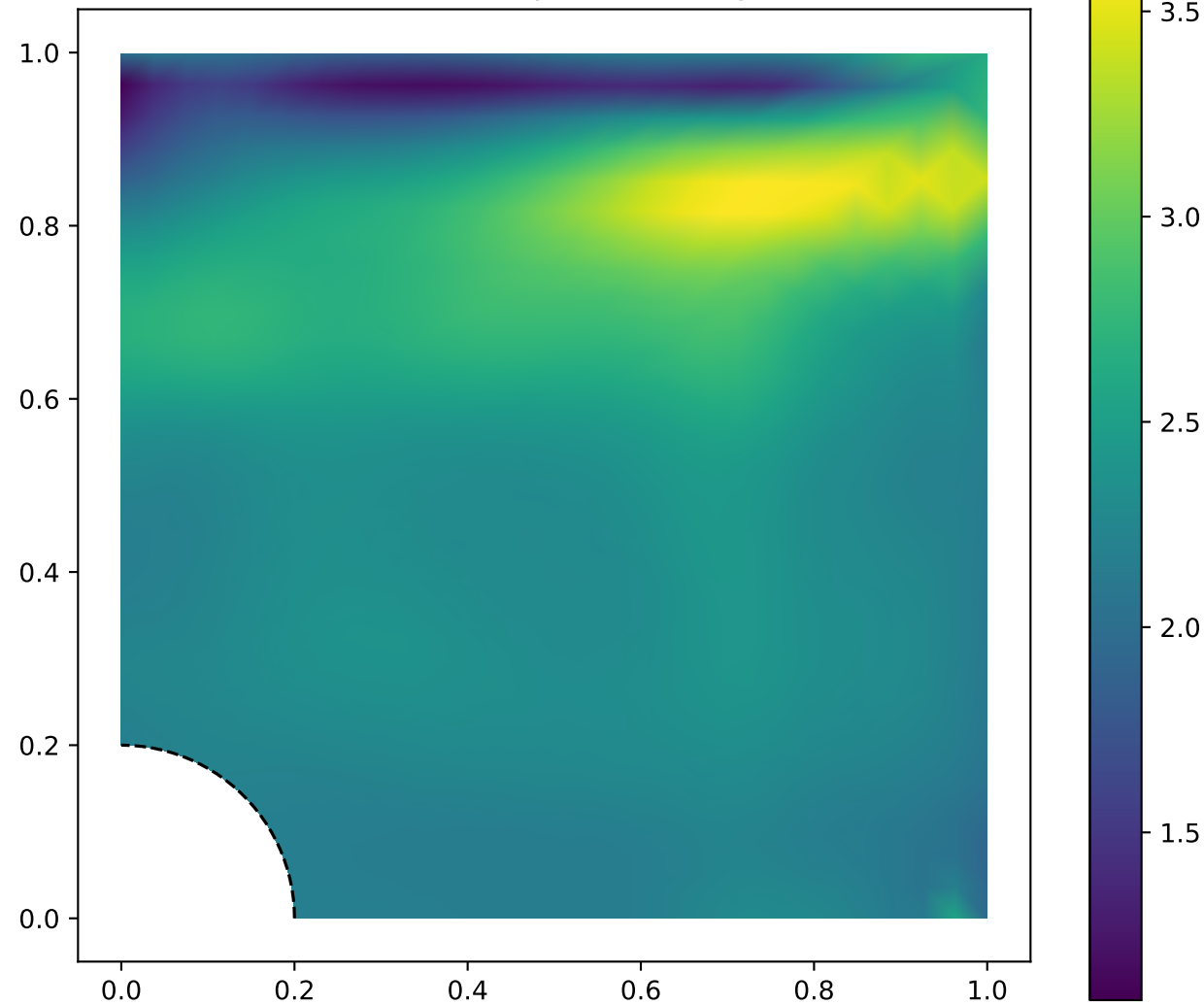
Plastic dissipation density
