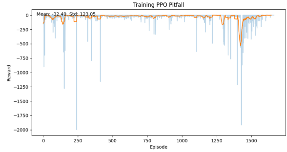
Fig. 1. Best baseline experiment for 5 000 000 timesteps
