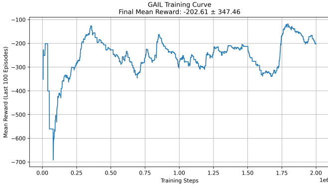
Fig. 3. Best baseline GAIL experiment for 2 000 000 timesteps
