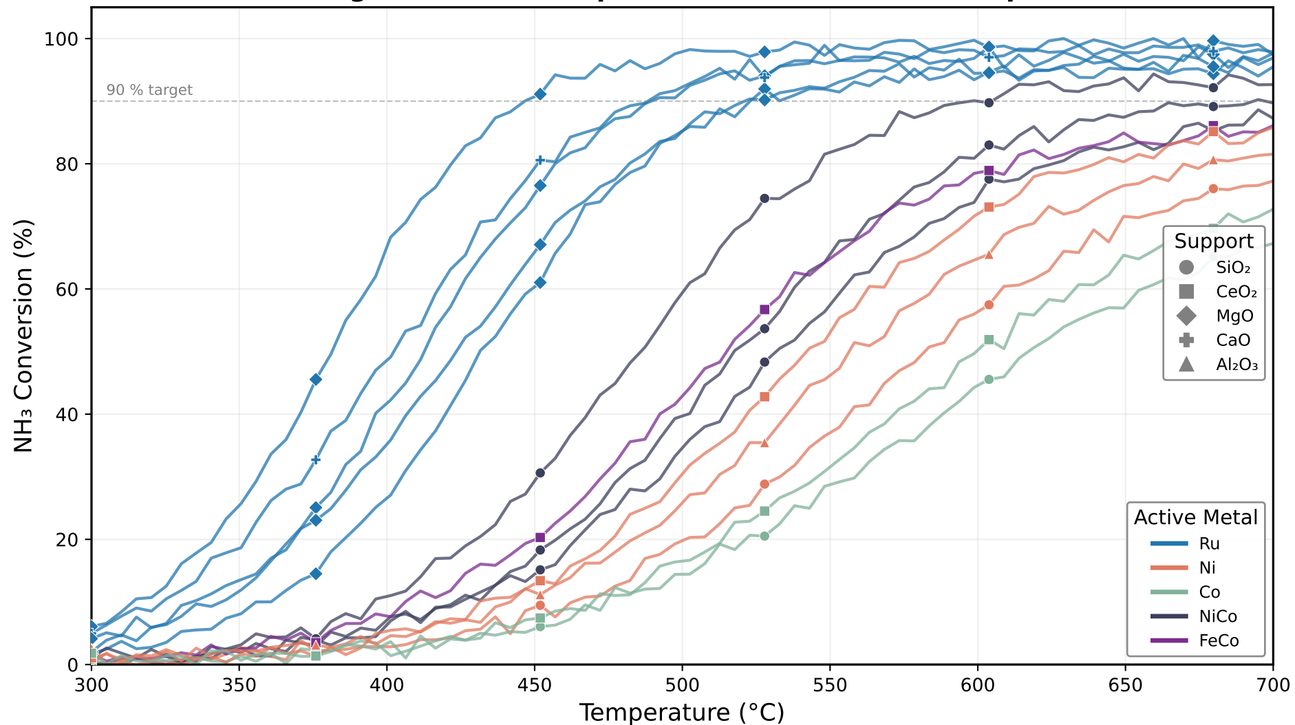
Figure 1 · Cross-Paper NH 3 Conversion Landscape
