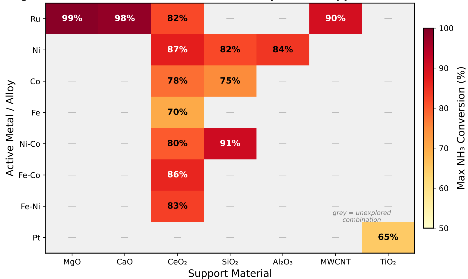
Figure 2 · Best \text{NH}_3 Conversion at 500 °C by Metal-Support Combination
